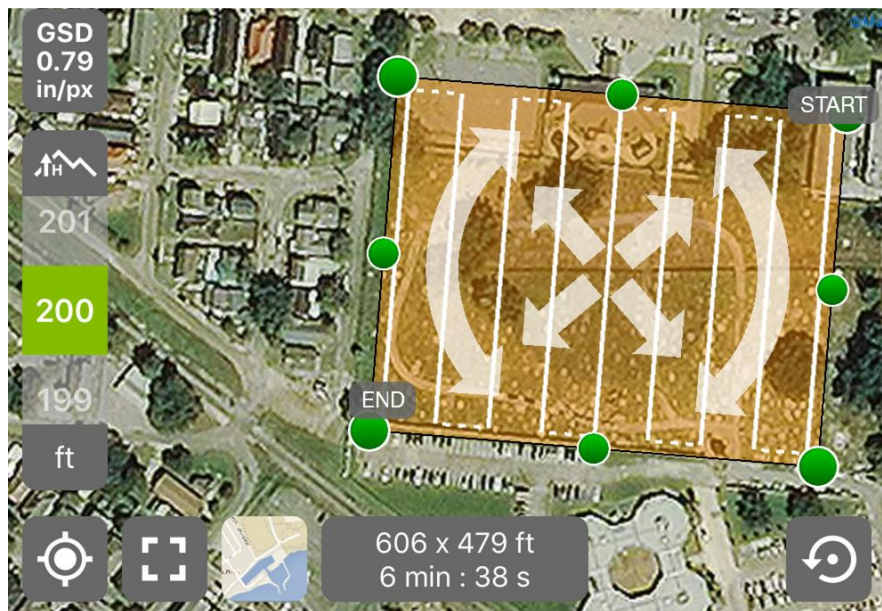
Figure 18. This screenshot was captured from the smart phone used to pilot the Unmanned Aerial System. The application used, Pix4d Capture, allows users to select a survey area and an altitude and then automatically generates a flight plan and triggers the UAS camera at the appropriate time in order to generate accurate spatial data.
